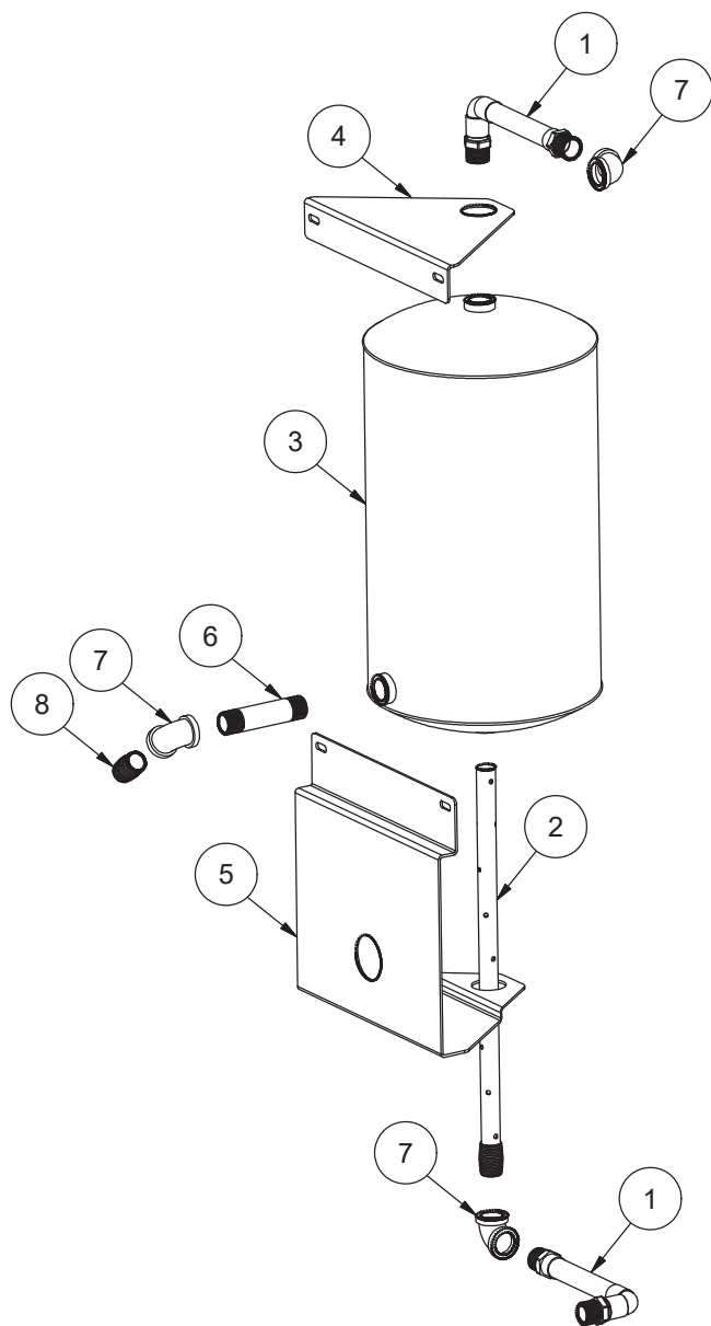
Complete CGP Tank Assembly 05700-002-45-05
