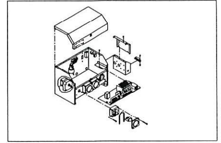
CONTROL BOX
